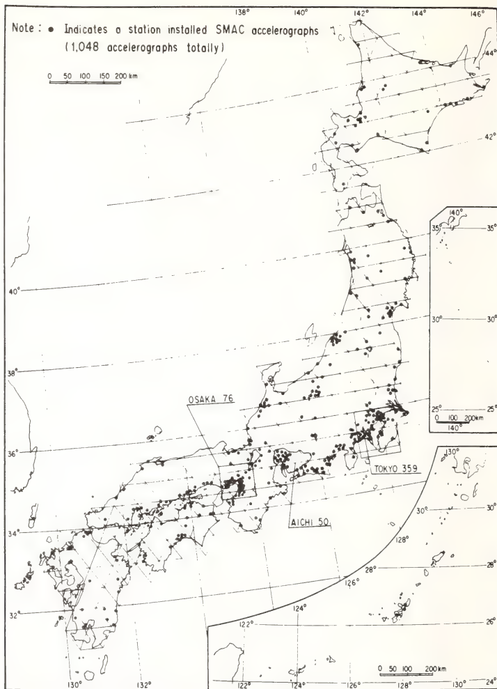
Fig. 1 Strong-Motion Observation Network in Japan as of March, 1976
